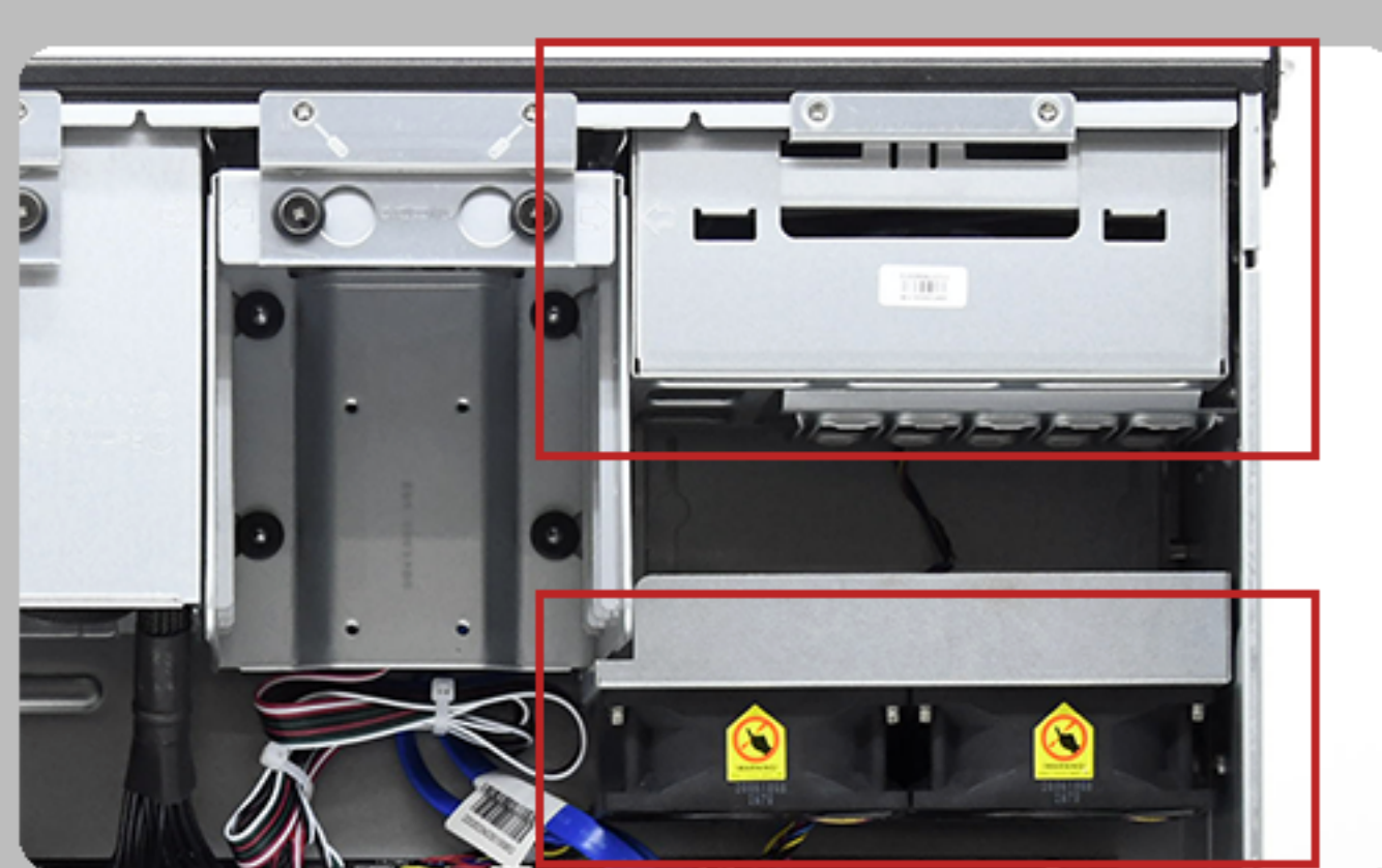
Easy-assembly front 120mm fan & Dual 80mm Cooling FAN for PCIEx card
